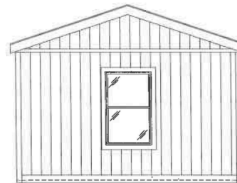
STD. FRONT ENDWALL
